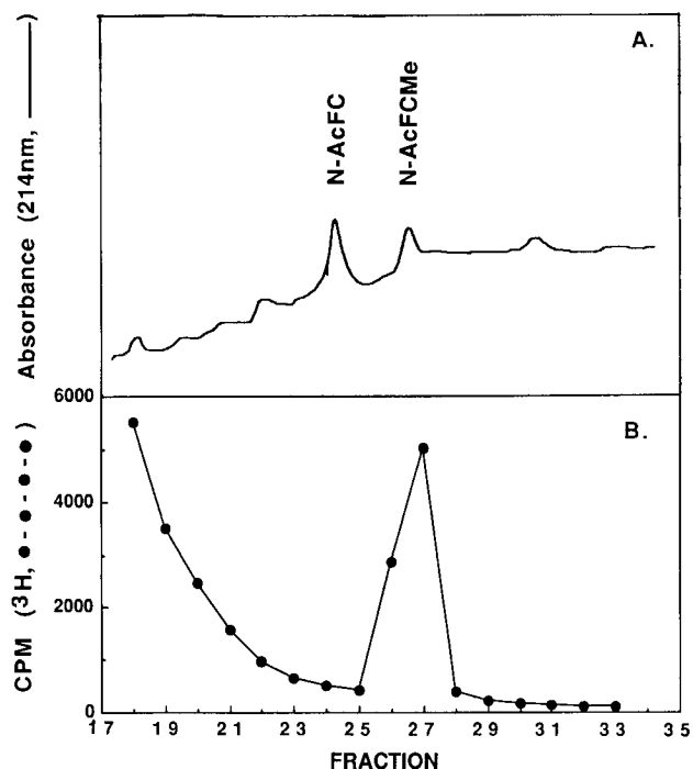
Fig. 2. Enzymatic formation of N -acetyl farnesyl cysteine [ 3 H]methyl ester ( N -AcFCMe) by the STE14 methyltransferase. N -AcFC was incubated in a reaction mixture containing 30 \mu l of 50 \mu M [ 3 H-methyl]AdoMet, 40 \mu l of crude membranes (0.71 mg protein) from BSG24 ( pTrpE-STE14 1-239 ) and 35 \mu l 100 mM Tris-HCl (pH 7.5). After incubation for 3 h at 37°C, 200 \mu l n -butanol was added and the sample was centrifuged at 13 000 g for 2 min. The n -butanol phase was retained and the aqueous layer was re-extracted with n -butanol as above. The combined n -butanol layers were evaporated to dryness and resuspended in 200 \mu l solvent A (solvent A is 0.1% trifluoroacetic acid in water, and solvent B is 0.1% trifluoroacetic acid-90% acetonitrile-9.9% water). (A) The total sample was fractionated on a C18 reversed phase column with a non-linear elution gradient of 0-70% solvent B/100-0% solvent A over 35 min and then up to 100% solvent B at 50 min at an initial flow rate of 1 ml/min. The unreacted substrate, N -AcFC, and its product, N -AcFCMe were detected by their UV absorption at 214 nm at 24-25 min and 26-27 min respectively; the peak at 24 min corresponds to 0.04 absorbance units. (B) One-minute fractions were collected and assayed for total radioactivity by counting 250 \mu l of each fraction in 10 ml of scintillation fluid. Nearly all of the radioactivity coelutes with the N -AcFCMe product. Aliquots (100 \mu l) of fractions corresponding to the N -AcFC and N -AcFCMe peaks were evaporated to dryness. An 80 \mu l aliquot of NaOH was added to each fraction and samples were directly assayed for methyl esters as described in Materials and methods. Quantitative amounts of [ 3 H]methanol, the expected product from base hydrolysis of a methyl ester, were released from the fraction corresponding to the 26-27 min peak (data not shown).
